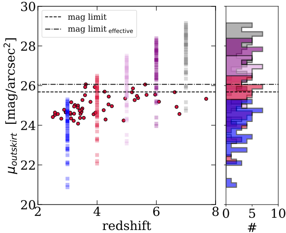
Fig. A.1. Surface brightness density as a function of redshift for the outskirts in our sample (red dots), along with the observed surface brightness shifted to different redshifts (squares), including the dimming effect of the universe. The magnitude detection limit is shown as a dashed line, while the effective magnitude limit is indicated by a dash-dotted line.
