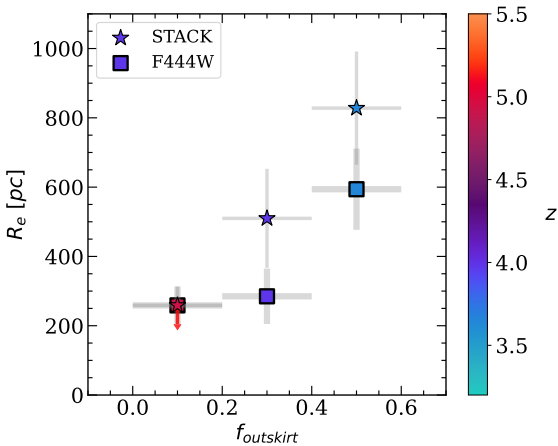
Fig. 10. Half light radii R_e as a function of f_{\text{outskirt}} . Stars correspond to the median R_e from stacking all the filters, and squares correspond to only F444W. The color bar shows the mean redshift in each f_{\text{outskirt}} bin.
