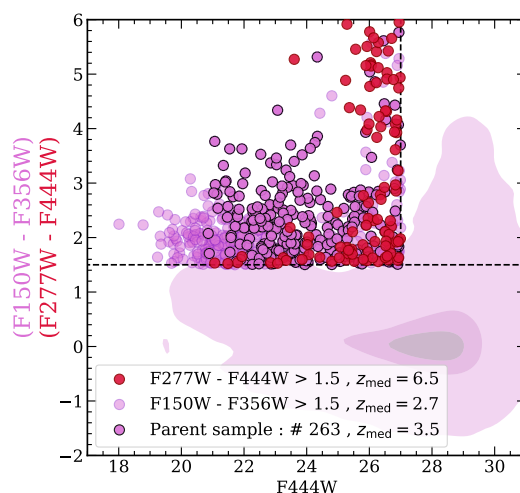
Fig. 1. Color magnitude diagram illustrating the parent sample : in purple we show the sources that respect the color-magnitude criterion, and black edges denotes the parent sample, respecting z > 2.5 . In red, we show the color-magnitude selection for the red color of LRDs F277W - F444W > 1.5 used in Akins et al. (2024), having a z_{\text{median}} \approx 6.5 . Red and purple contours represent all CEERS sources at 25%, 50% and 80% levels shown for F150W-F356W.
