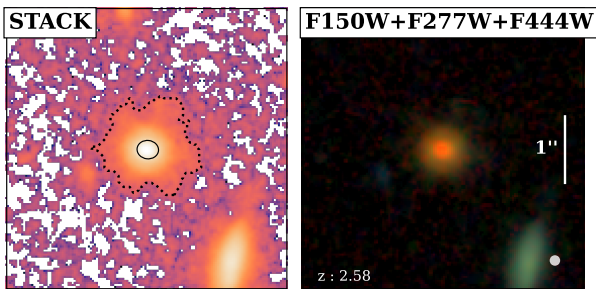
Fig. 2. Example illustrating the definition of the outskirts and inner regions. Left panel: stacked image combining all JWST bands, defined as \text{STACK} = F115W + F150W + F200W + F277W + F356W + F410M + F444W , using PSF-matched data. The dotted line shows the segmentation map, while the solid line traces the ellipse with a semi-major axis of 0.16'' = 2\text{HWHM} . Right panel: color composite image using F150W (blue), F277W (green), and F444W (red). The white circle indicates the PSF FWHM beam at F444W. As expected, the galaxy exhibits a centrally concentrated red emission and a bluer, more extended periphery.
