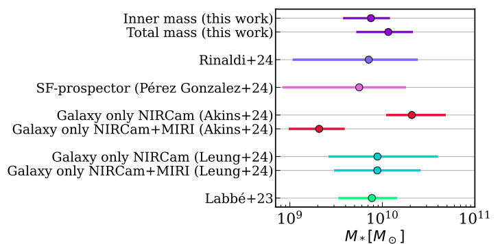
Fig. 5. Mass distribution for several samples of LRDs from previous works, assuming only a stellar model, from Rinaldi et al. (2024); Pérez-González et al. (2024); Akins et al. (2024); Leung et al. (2024); Labbé et al. (2023). This sample is visible in purple for both the inner part and the total mass.
