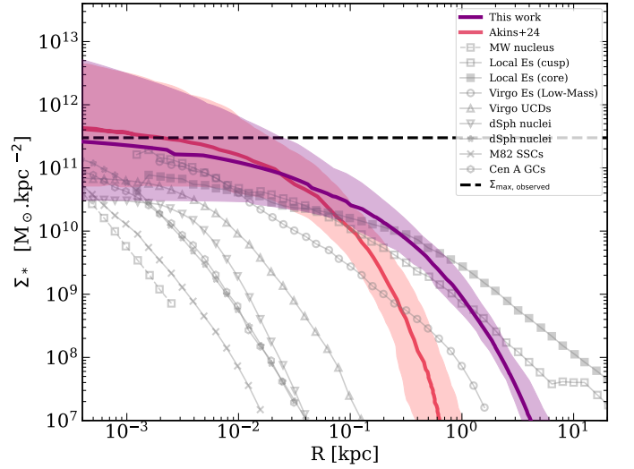
Fig. 7. Stellar mass density profiles for our sample using only resolved galaxies in purple. In red the profile inferred by Akins et al. (2024) assuming only a stellar model. We also add dense cores from Hopkins et al. (2010) and Grudić et al. (2019).
