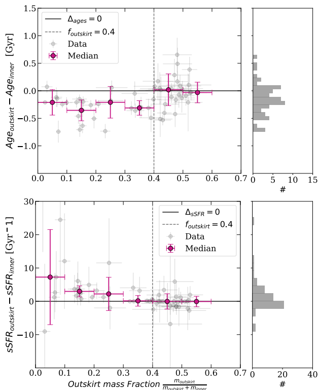
Fig. 14. Differences of Ages and sSFR between the outskirts and inner part as a function of the outskirts mass fraction f_{\text{outskirt}} . The data are shown in grey with the median profile in pink. For each distribution, the black solid line refers to no radial changes between the inner/outskirt part.
