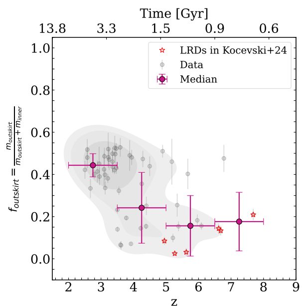
Fig. 9. Outskirts mass fraction as a function of redshift. Gray dots represent the data, while gray contours illustrate their distribution at 0.25, 0.5 and 0.75 levels. The median is shown as a purple circle, with each point computed in bins of \Delta z = 1 . Vertical error bars indicate the standard deviation, while horizontal bars represent the width within each bin. Red stars refer to the LRDs also in Kocevski et al. (2025) .
