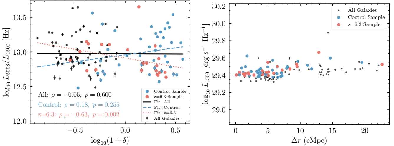
Figure 4. Left: [O III]-to-UV luminosity ratio ( \log_{10}(L_{5008}/L_{1500}) ) versus local overdensity, estimated with a k = 5 near-neighbor metric in 3D over the full sample of 130 emitters ( 5.3 < z < 6.9 ) and normalized to the field average. The combined control sample (foreground z \approx 6.2 plus background z \approx 6.8 ; blue hexagons) shows a weak positive trend ( \rho = 0.18 , p = 0.255 ), while the z \approx 6.3 near-QSO sample (red circles) shows a negative trend ( \rho = -0.63 , p = 0.002 ). The full sample shows no significant correlation ( \rho = -0.05 , p = 0.600 ). These patterns indicate that the quasar-distance dependence is unlikely to be driven by local overdensity alone. Right: Rest-frame UV luminosity ( \log_{10} L_{1500} ) as a function of transverse distance \Delta r from J0100+2802. Both the near- z_{\text{QSO}} and control samples show no significant trend with distance, with a typical scatter of about 0.2 dex. The y-axis span (in dex) matches Figure 2 (right) for visual comparison.
