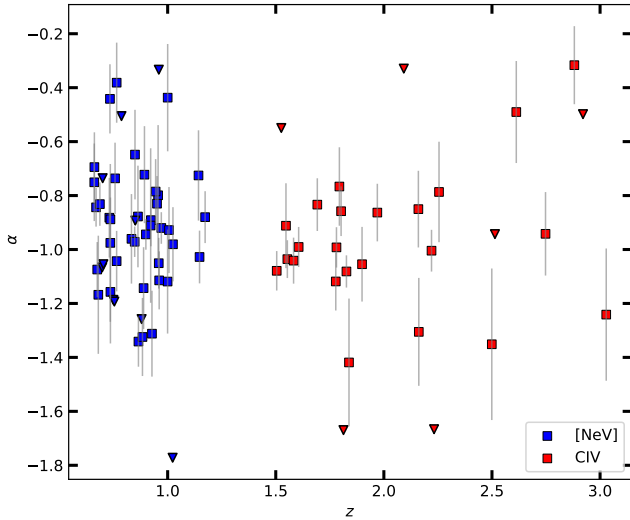
Figure 11. Radio spectral index as function of redshift for the [Ne v] (Blue) and for the C iv (Red) AGN. The radio spectral index is measured using the 3 GHz flux from Smolčić et al. (2017a) and MIGHTEE flux at the effective frequency of each source (median \nu_{\text{eff}} = 1.24 GHz). Triangles denote upper limits, i.e. sources with MIGHTEE detection but undetected by VLA.
