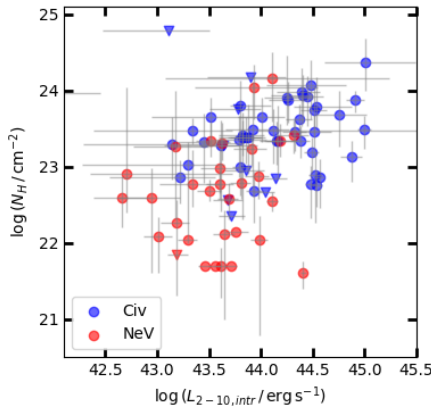
Figure 2. Obscuration as a function of the intrinsic 2 – 10 keV luminosity for X-ray detected sources in the C iv (blue) and [Ne v] samples (red). The grey lines are the associated 90% uncertainties. The triangles denote upper limits on the amount of obscuration due to the difficulties in properly constraining it in the case of spectra with a low number of photon counts.
