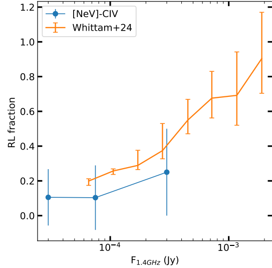
Figure 10. Comparison of the radio loudness fraction as a function of the source radio flux between this work (blue) and the central 0.86 \text{ deg}^2 of the COSMOS field by Whittam et al. (2024, orange). In both cases, we computed the flux densities at 1.4 GHz by rescaling the measured ones assuming a spectral index of \alpha = 0.7 .
