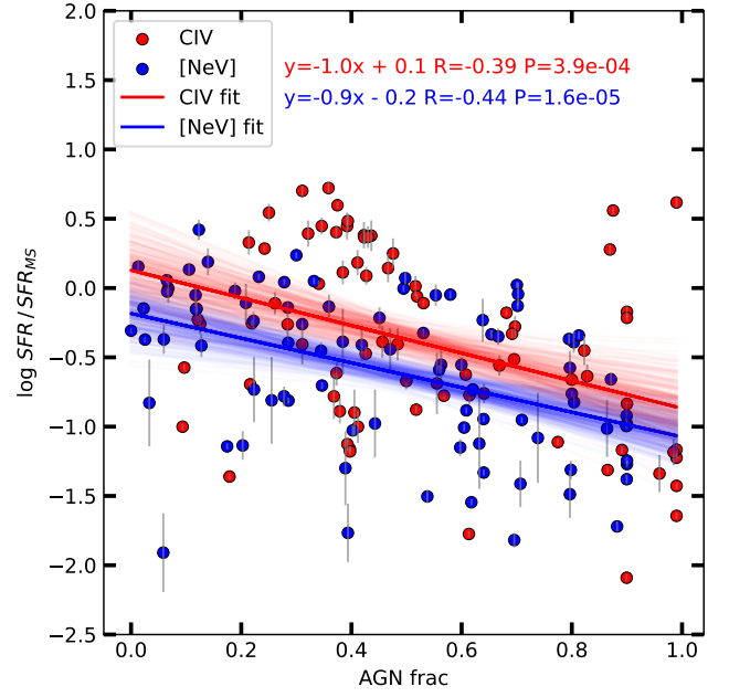
Figure 6. Offset with respect to the MS as a function of the AGN fraction for the [Ne v] (blue) and C iv (red) samples. The solid lines are the best-fit from linear regression analysis, the light lines are obtained by bootstrapping the samples 300 times. R and P refer to the Pearson correlation coefficient and P-value, respectively.
