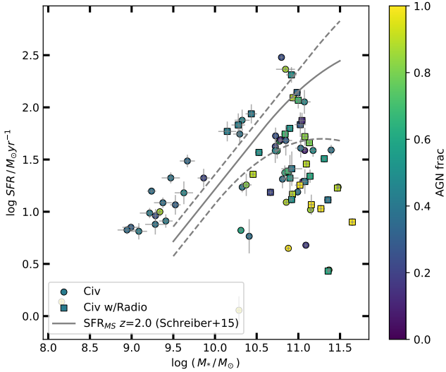
Figure 5. Comparison of the positions of the C iv sample in the SFR - M_* plane. The squares represent the C iv sources detected in the radio band (either MeerKAT or VLA), while the circles represent those without radio detection. The colour code denotes the 1 - 1000 \mu\text{m} AGN fraction. The grey solid line is the Schreiber et al. (2015) MS at the mean redshift of the sources, the grey dashed lines its 1 \sigma dispersion.
