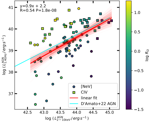
Figure 9. AGN 1.4 GHz luminosity versus rest frame 2 – 10 keV luminosity, for the [Ne v] (circle) and C iv (square) sources with both X-ray and radio detection. The colour code indicates the optical radio loudness R_O . The dark red line is the best-fit from linear regression analysis, and the light red lines are obtained by bootstrapping the sample 300 times. The cyan line is the same correlation found by D’Amato et al. (2022) for AGN in the J1030 field. R and P refer to the Pearson correlation coefficient and P-value, respectively.
