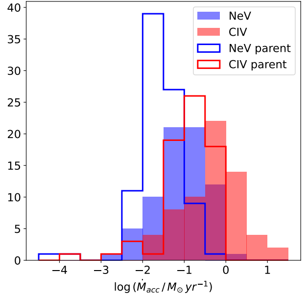
Figure 13. Distribution of the BH accretion rates of the [Ne v]-C iv ‘‘analogue sample’’ and of their ‘‘parent samples’’. Blue histograms are for the [Ne v] AGN, red ones refers to the C iv AGN. The ‘‘analogue sample’’ is composed of SIMBA galaxies matched in redshift, stellar mass, SFR, and \dot{M}_{\text{BH}} to the [Ne v] and C iv sources. The ‘‘parent sample’’ has been similarly built without matching \dot{M}_{\text{BH}} , representing the average galaxy population. It is easy to see that our selection picks out sources in a stronger-than-average phase of accretion.
