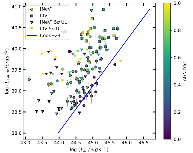
Figure 12. 1.4 GHz radio luminosity as function of the SF-related 1-1000\mu\text{m} IR luminosity. The colour code indicates the AGN fraction in the 1-1000\mu\text{m} wavelength range. L_{1.4\text{GHz}} is computed from the MIGHTEE 5.2'' total flux, assuming spectral index \alpha = -0.7 . The triangles and arrows indicate the 5\sigma upper limits on the radio luminosity, calculated at each source position from the MIGHTEE 5.2'' sensitivity map, for the [Ne v] and C iv sources, respectively. L_{\text{IR}}^{\text{SF}} is an output of the SED-fitting procedure, and it takes into account only the IR emission due to SF processes, i.e. without any AGN contribution. The blue line refers to the Cook et al. (2024) IR-radio correlation in case of pure SF processes.
