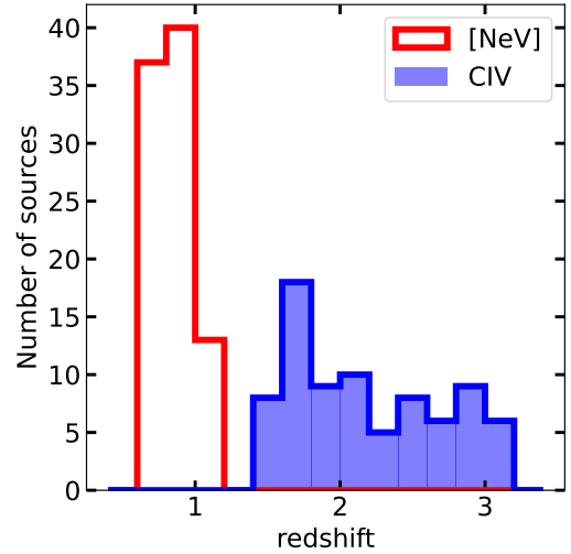
Figure 1. Redshift distribution of the C iv- (blue) and [Ne v]- (red) selected AGN. The redshift distribution is primarily determined by the requirement that the [Ne v]3426 and C iv1549 emission lines fall within the wavelength coverage of VIMOS.
