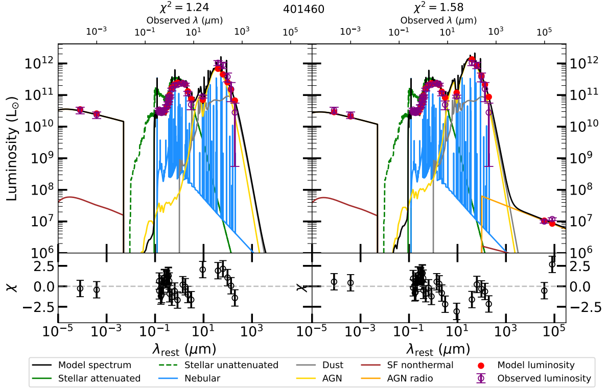
Figure C1. Comparison of the best-fit SED for source zCOSMOS ID401460 with (left panel) and without (right panel) the inclusion of the radio band photometry. The purple points are the observed photometry, the red ones refer to the best-fit model luminosity. The black line is the best-fit model, composed of the stellar attenuated emission (green continuous line), the nebular emission (blue), the dust emission (grey), the AGN emission in the optical-IR (yellow), the AGN emission at radio and X-ray wavelengths (orange), and the SF-related emission at the same bands (brown). The dashed green line is the intrinsic (i.e. extinction-corrected) stellar emission. For this source, having already a good IR and X-ray coverage, the addition of the radio band to the SED fitting does not significantly change the results.
