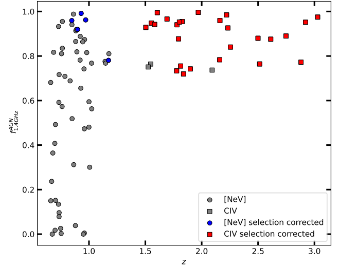
Figure 8. Fraction of the 1.4 GHz radio luminosity that can be ascribed to AGN-related processes ( f_{1.4\text{GHz}}^{\text{AGN}} ) versus redshift for the [Ne v] (circle) and C iv (square) sources. Blue (Red) points are [Ne v] (C iv) “selection corrected” sources, i.e., those with AGN luminosity L_{1.4\text{GHz}} > 10^{40} erg/s that can be detected in the entire redshift range. The lower number of [Ne v] AGN with L_{1.4\text{GHz}} > 10^{40} erg/s is due to the smaller comoving volume.
