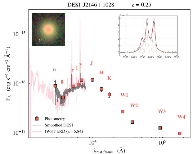
Fig. 1: Multi-wavelength view of an LRD analogue at z = 0.25 . Main panel: Rest-frame SED showing archival photometry (red squares) and the smoothed DESI spectrum (black line). For comparison, the rest-frame JWST/NIRSpec PRISM spectrum of a high-redshift LRD is over-plotted in pink. Top-left inset: DESI Legacy Imaging Surveys grz -composite image (Dey et al. 2019) showing the compact morphology. Top-right inset: Zoomed-in rest-frame DESI spectrum and fitting models of the H\alpha region.
